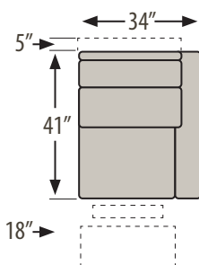
FLYN-85: RAF Motorized Recliner with Headrest
