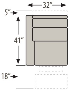
FLY2-84: LAF Motorized Recliner with Headrest
